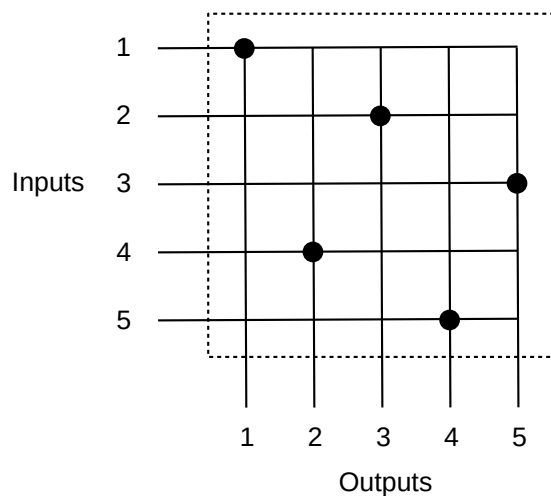
5x5 crossbar with 5 parallel connections 1 → 1, 2 → 3, 3 → 5, 4 → 2, 5 → 4
